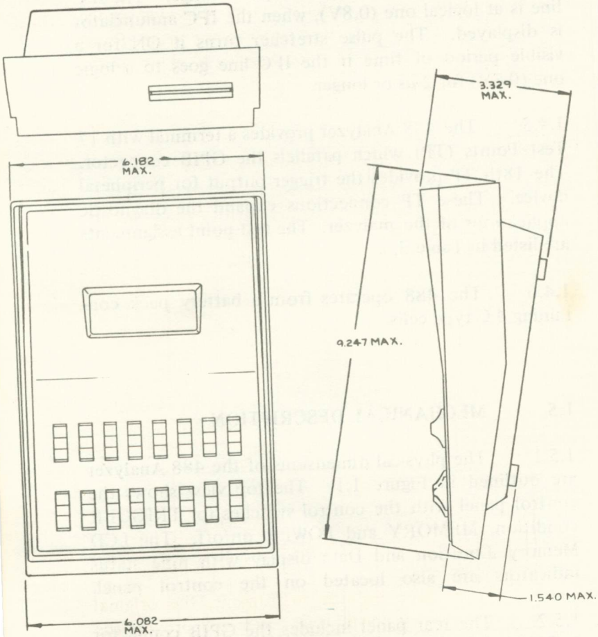
Figure 1.1 - Dimensional Outline
